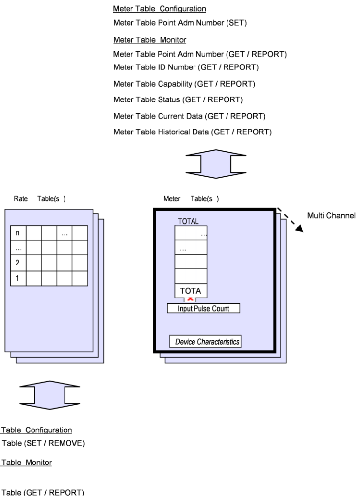
Figure 18. Data model for Adv. Import / Export Meter with rates
